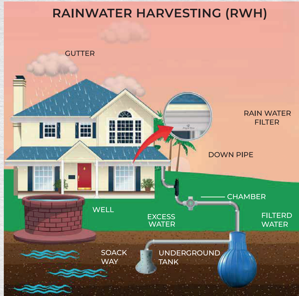
Underground Soak Away
